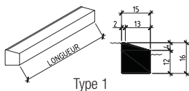
Type 1
